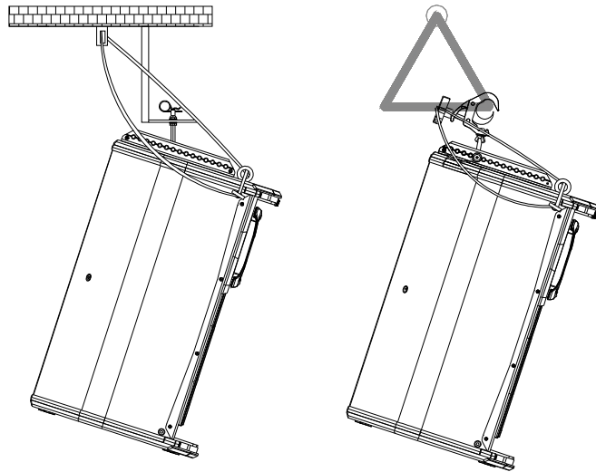
Fig. 20. RB-L and RB-L/GT flying bar for S15P
