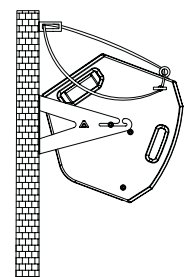
HORIZONTAL WALL-MOUNT UB-L + SC-15
