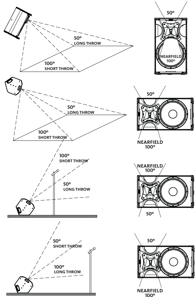
VERTICAL COLUMN-MOUNT HR-LU + SC-15
